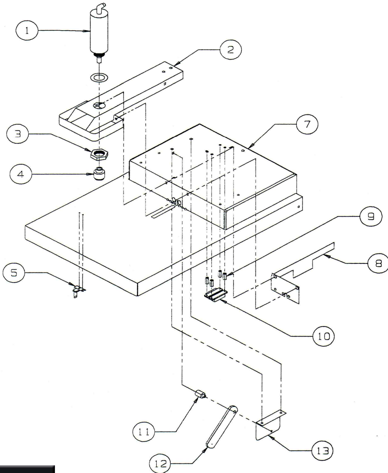
TSM-31/TSM-35 TOP ASSEMBLY DETAIL 3 OF 5
