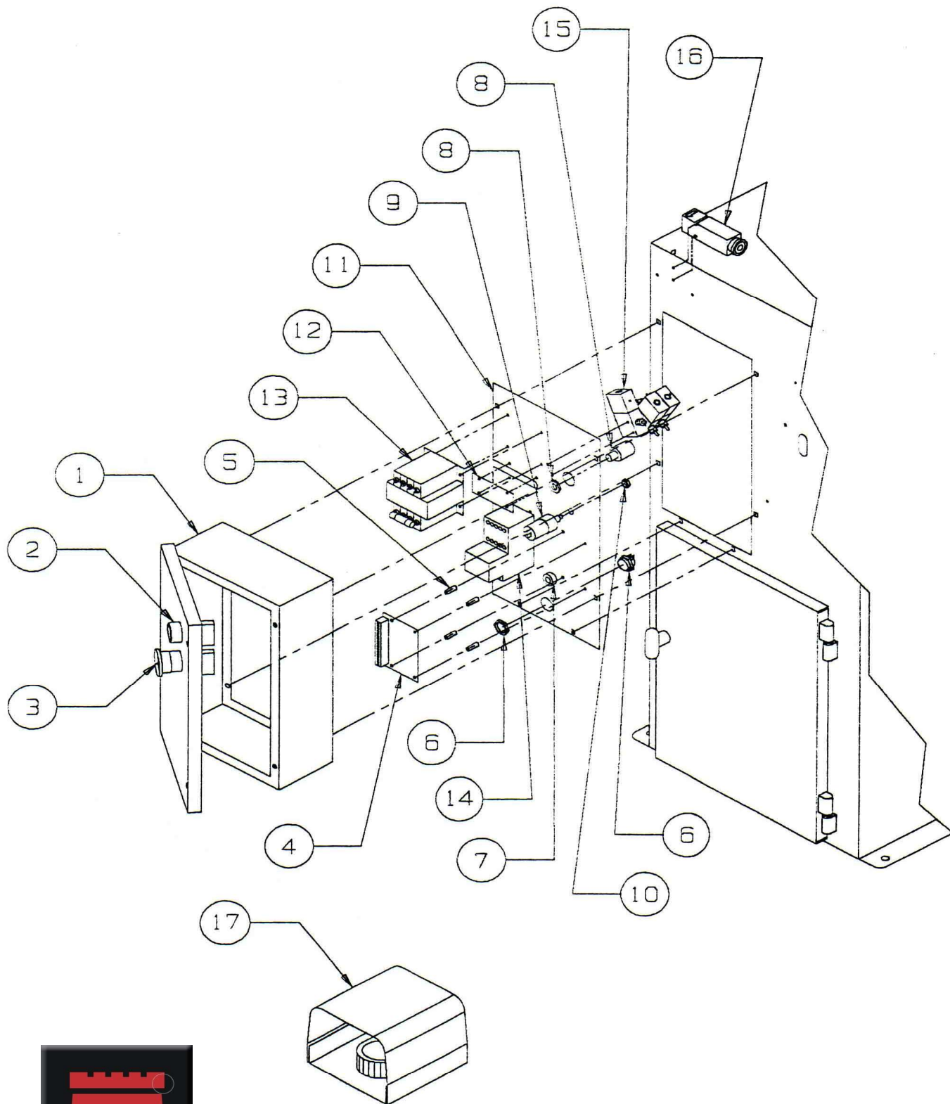
TSM-31/TSM-35 CONTROL PANEL DETAIL
