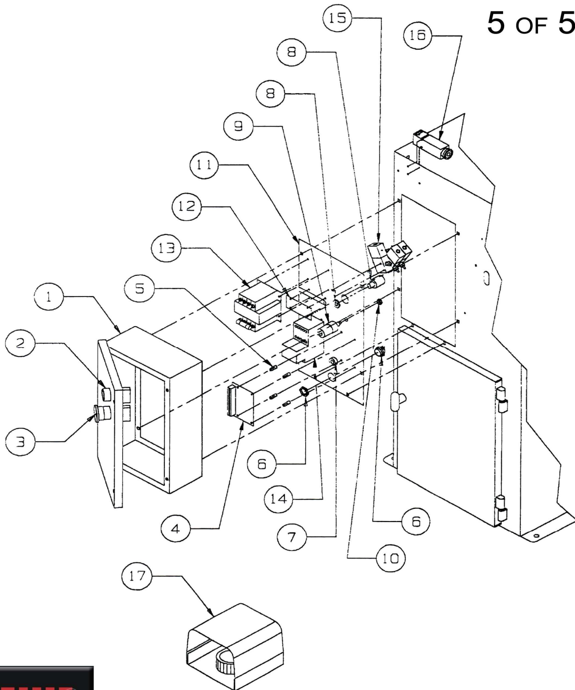
TSM-31/TSM-35 CONTROL PANEL DETAIL
