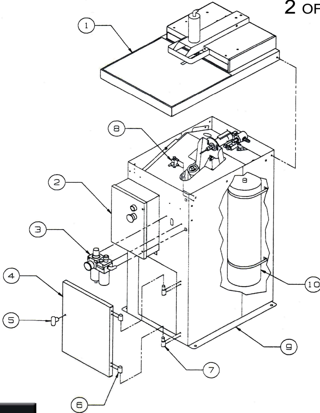
TSM-31/TSM-35 CASE ASSEMBLY DETAIL
