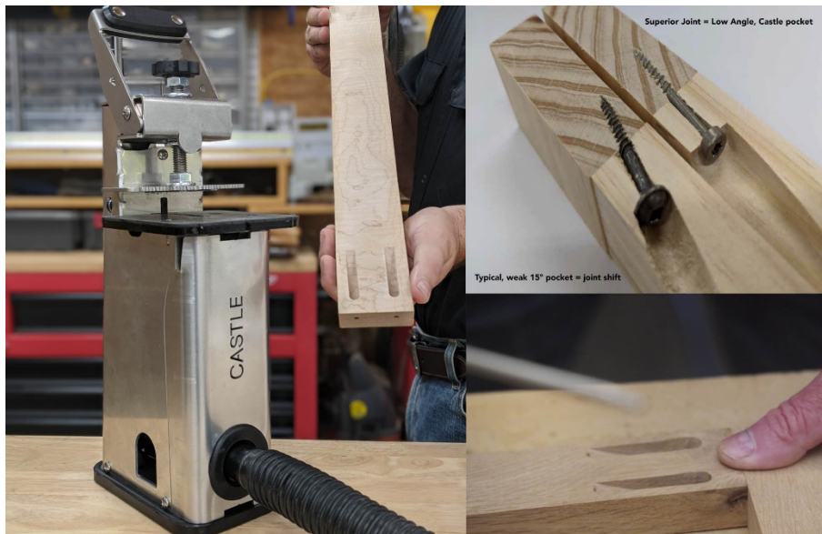
The new Castle 110 – professional pocket hole joinery in a small, portable, adjustable machine.
